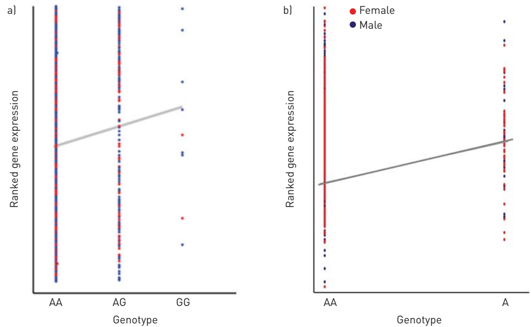
FIGURE 4 Expression quantitative trait loci (eQTL) identified for COMMD10 single nucleotide polymorphisms (SNPs) rs10036292 in a) blood ( p=3.68 \times 10^{-4} ) and b) lung tissue (meta-analysis p=5.24 \times 10^{-9} ). Order on x-axis is from nonrisk homozygote to heterozygote and risk homozygote. Note in the lung tissue dataset, the risk homozygotes were not present.
