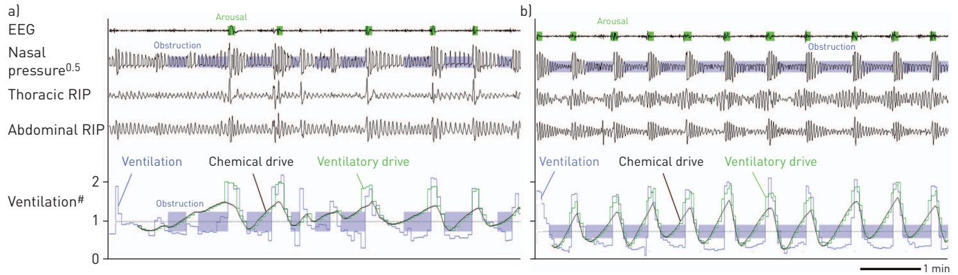
FIGURE 3 Estimating loop gain using diagnostic polysomnography. Example traces illustrate epochs with a) relatively low loop gain (response to a 1\text{-cycle}\cdot\text{min}^{-1} disturbance ( LG_1=0.6 ) and b) relatively high loop gain ( LG_1=1.1 ). Note that ventilatory drive (chemical drive + response to arousal) closely fits ventilation during periods of unobstructed airflow. Loop gain determines the increase in chemical drive in response to the reduction in ventilation. EEG: electroencephalogram; RIP: respiratory inductance plethysmography. #: normalised.
