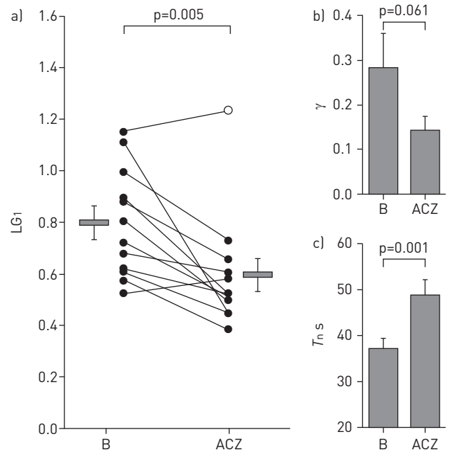
FIGURE 6 Detecting the reduction in loop gain with acetazolamide (ACZ). a) Reduction in loop gain (response to a 1-cycle·min -1 disturbance (LG1)) with ACZ versus baseline (B). b) Reduced ventilatory response to arousal ( \gamma ), as a fraction of mean ventilation, with ACZ. c) The feedback system's natural cycling period ( T_n ) rose with ACZ ( i.e. feedback was more sluggish). Note that in one subject, LG1 and other variables were not measured from the obstructive sleep apnoea pattern on ACZ due to insufficient obstructive events. The open circle represents a patient whose loop gain unexpectedly rose with ACZ as confirmed with the continuous positive airway pressure drop method. Data are presented as mean \pm SEM.
